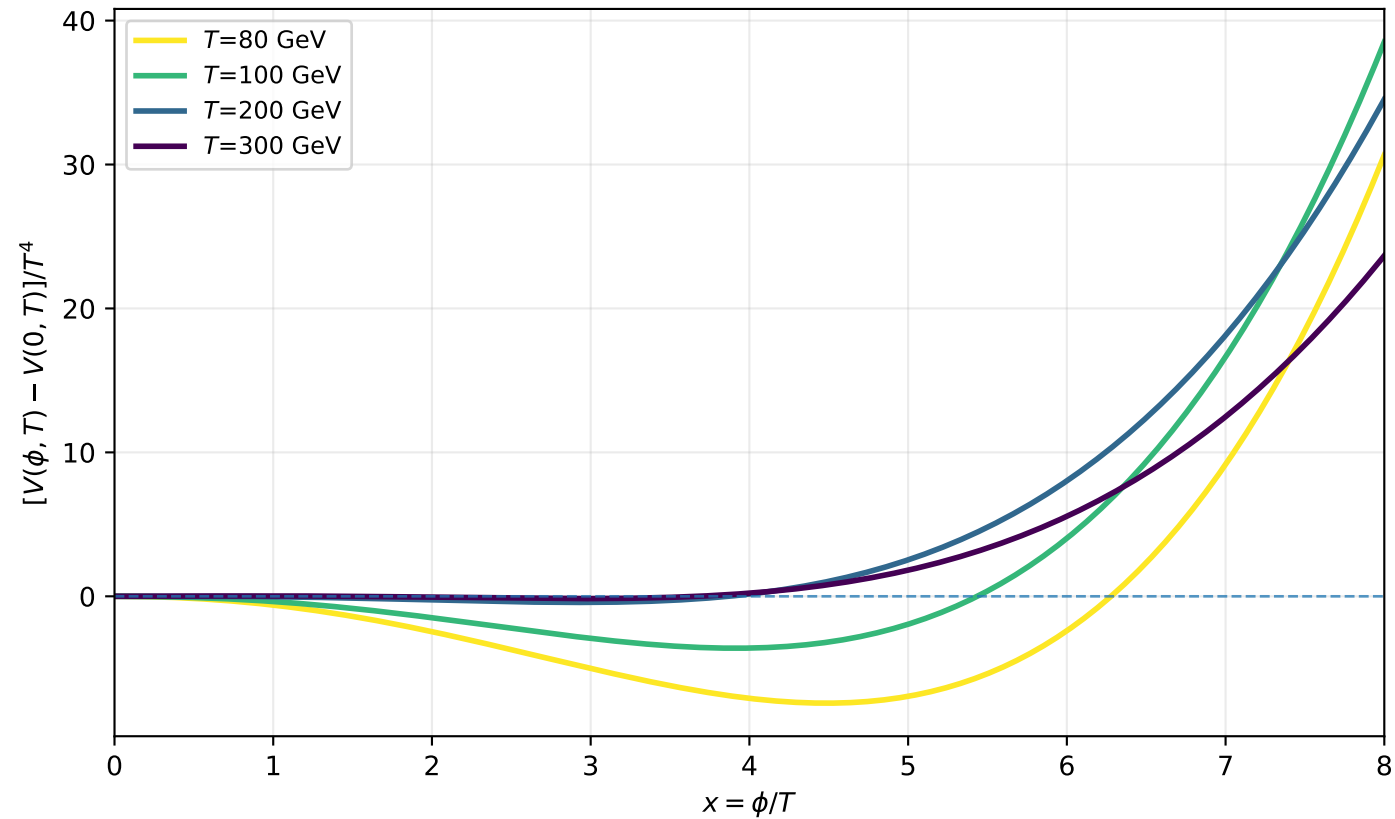
Example B6: dimensionless potential in \phi/T
