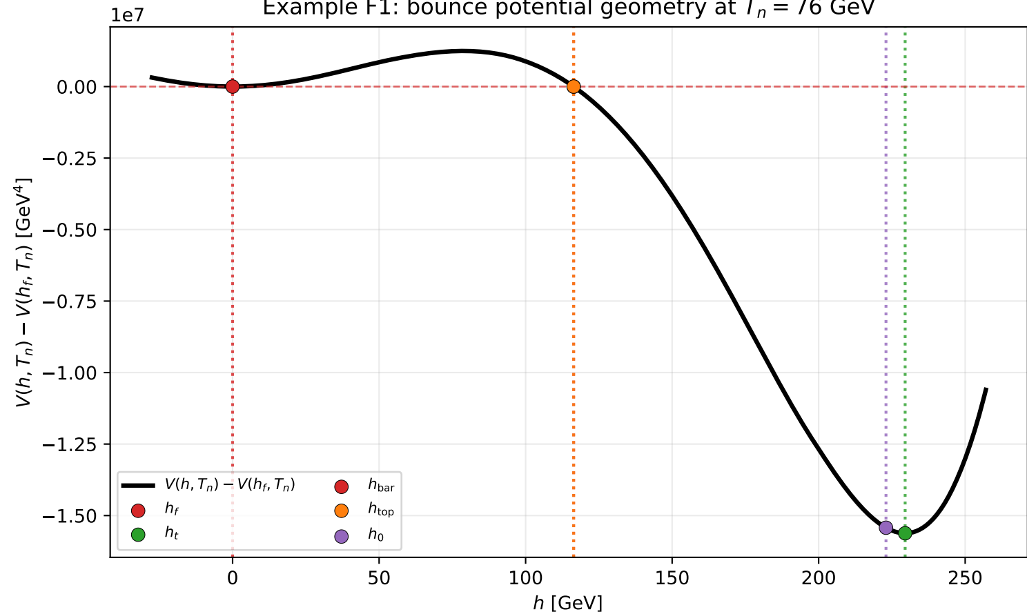
Example F1: bounce potential geometry at T_n = 76 GeV
