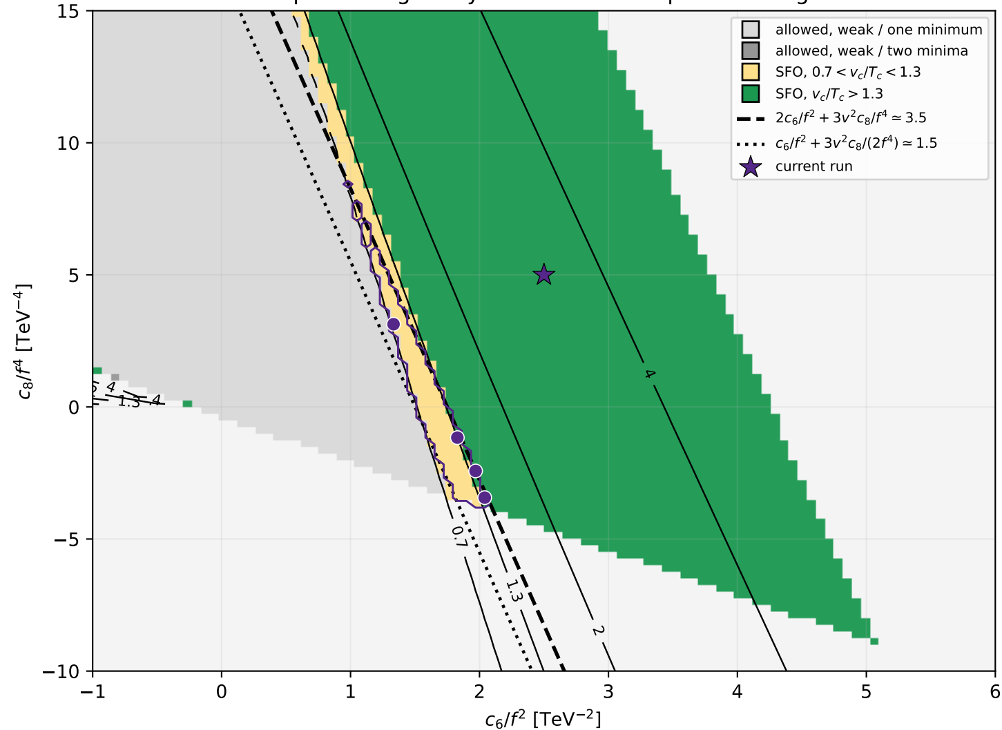
Example D1: Fig. 2-style mean-field map and scan guide
