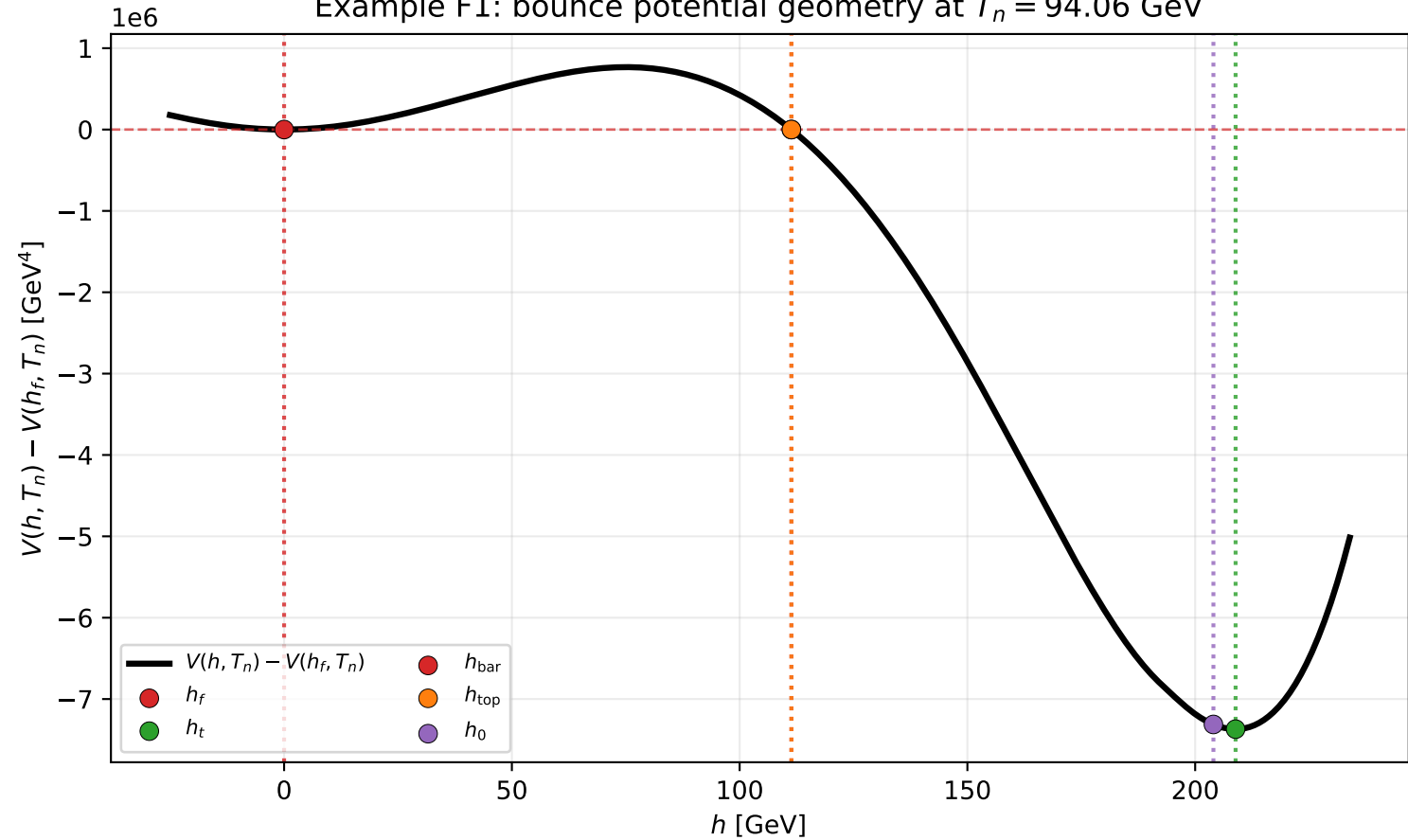
Example F1: bounce potential geometry at T_n = 94.06 GeV
