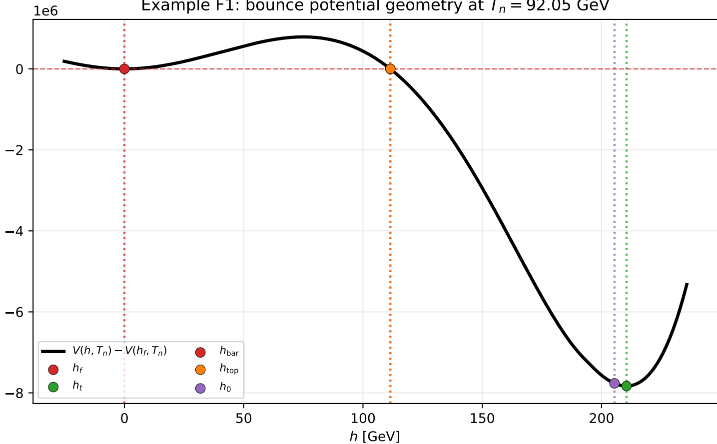
Example F1: bounce potential geometry at T_n = 92.05 GeV
