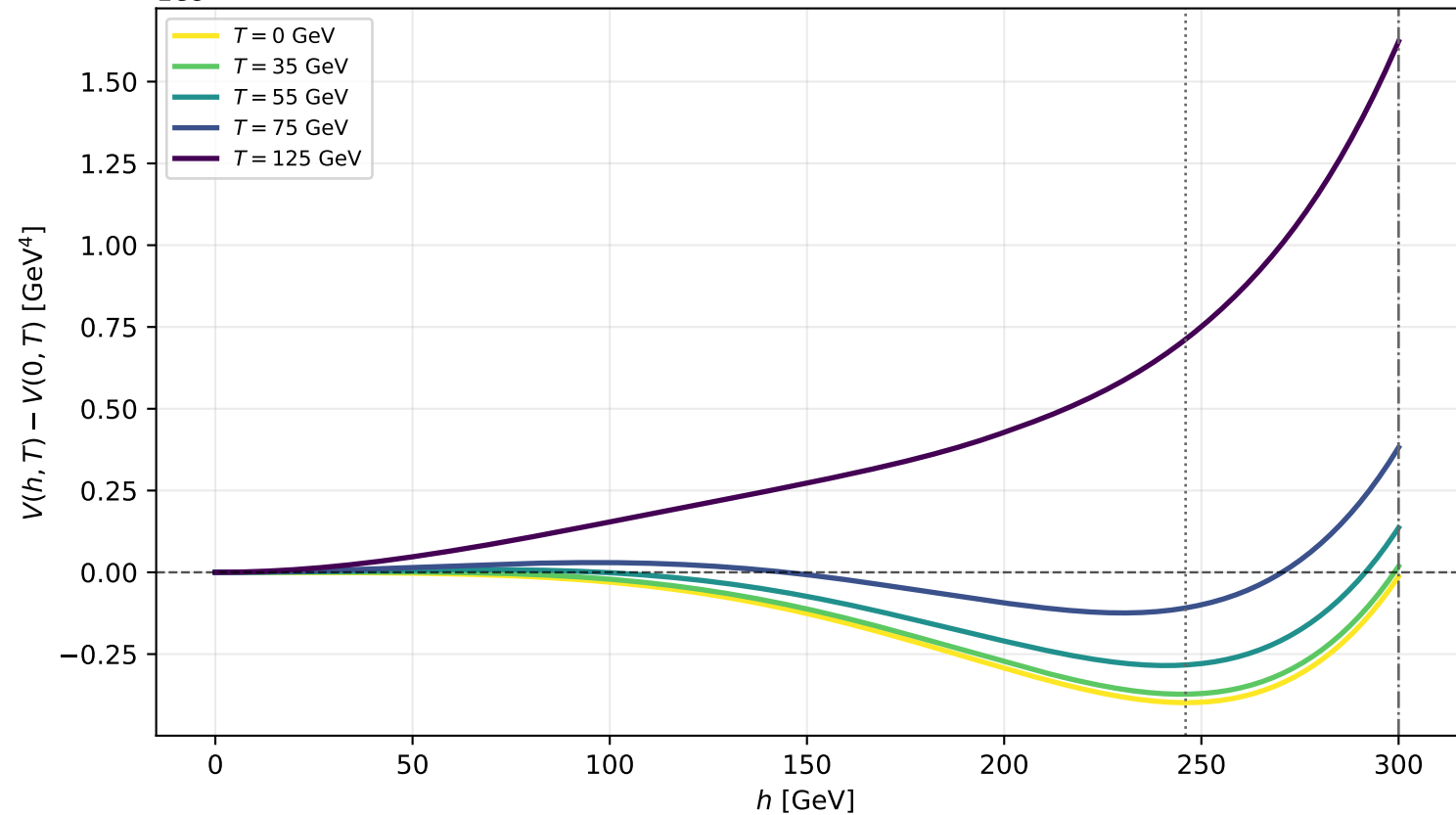
1e8 Example C1: quick finite-temperature potential shapes (diagnostic only)
