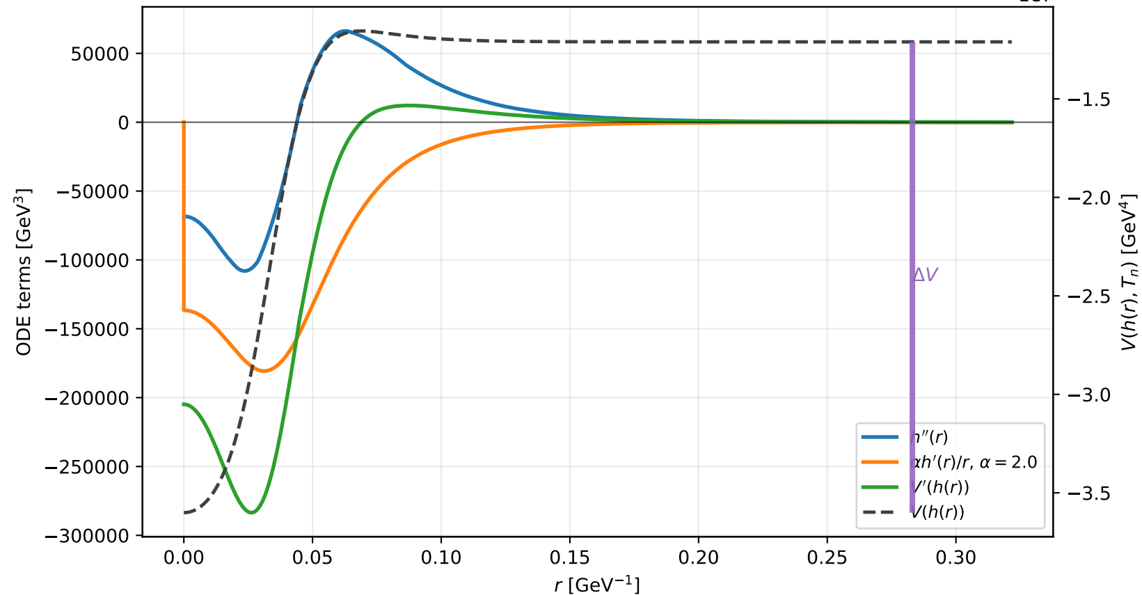
Example F7: bounce equation terms at T_n = 43.95 GeV
