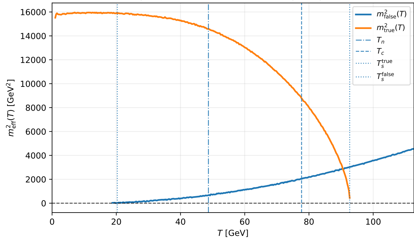
Example E5: curvature masses along the phases
