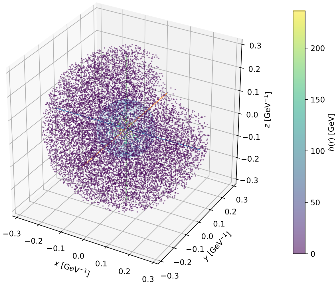
Example F5: 3D bubble profile at T_n = 68.62 GeV
