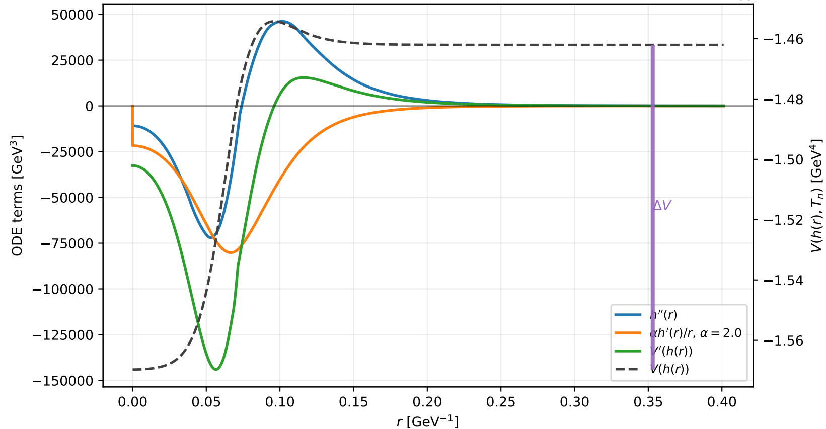
Example F7: bounce equation terms at T_n = 85.16 GeV
