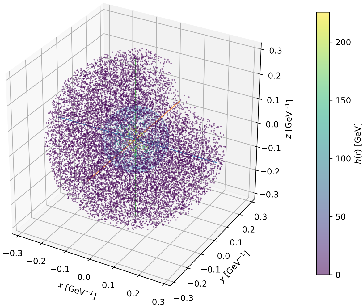
Example F5: 3D bubble profile at T_n = 80.64 GeV
