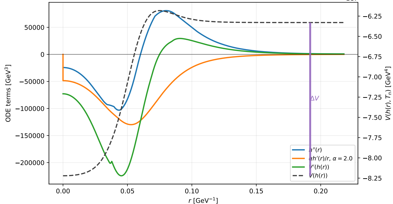
Example F7: bounce equation terms at T_n = 70.63 GeV
