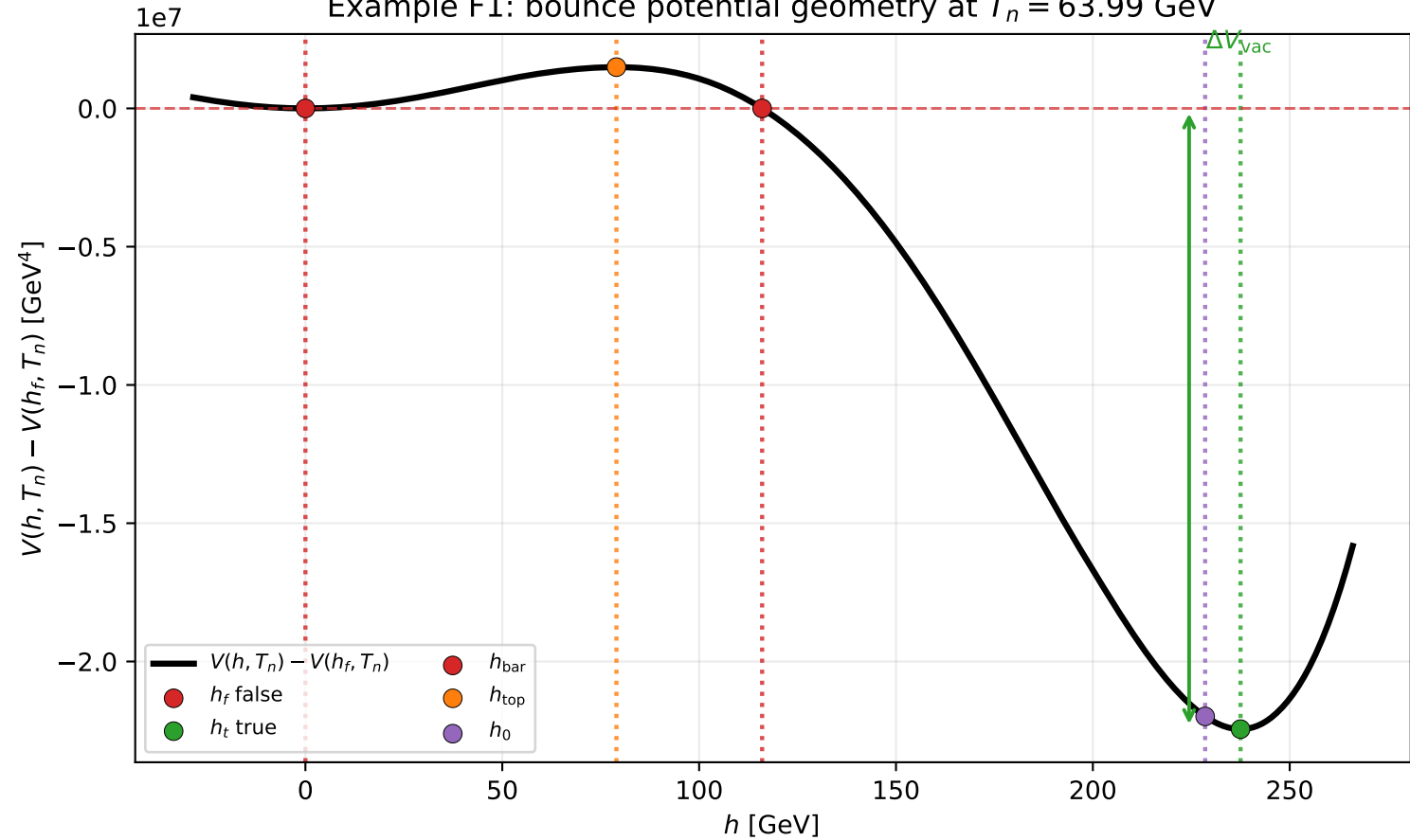
Example F1: bounce potential geometry at T_n = 63.99 GeV
