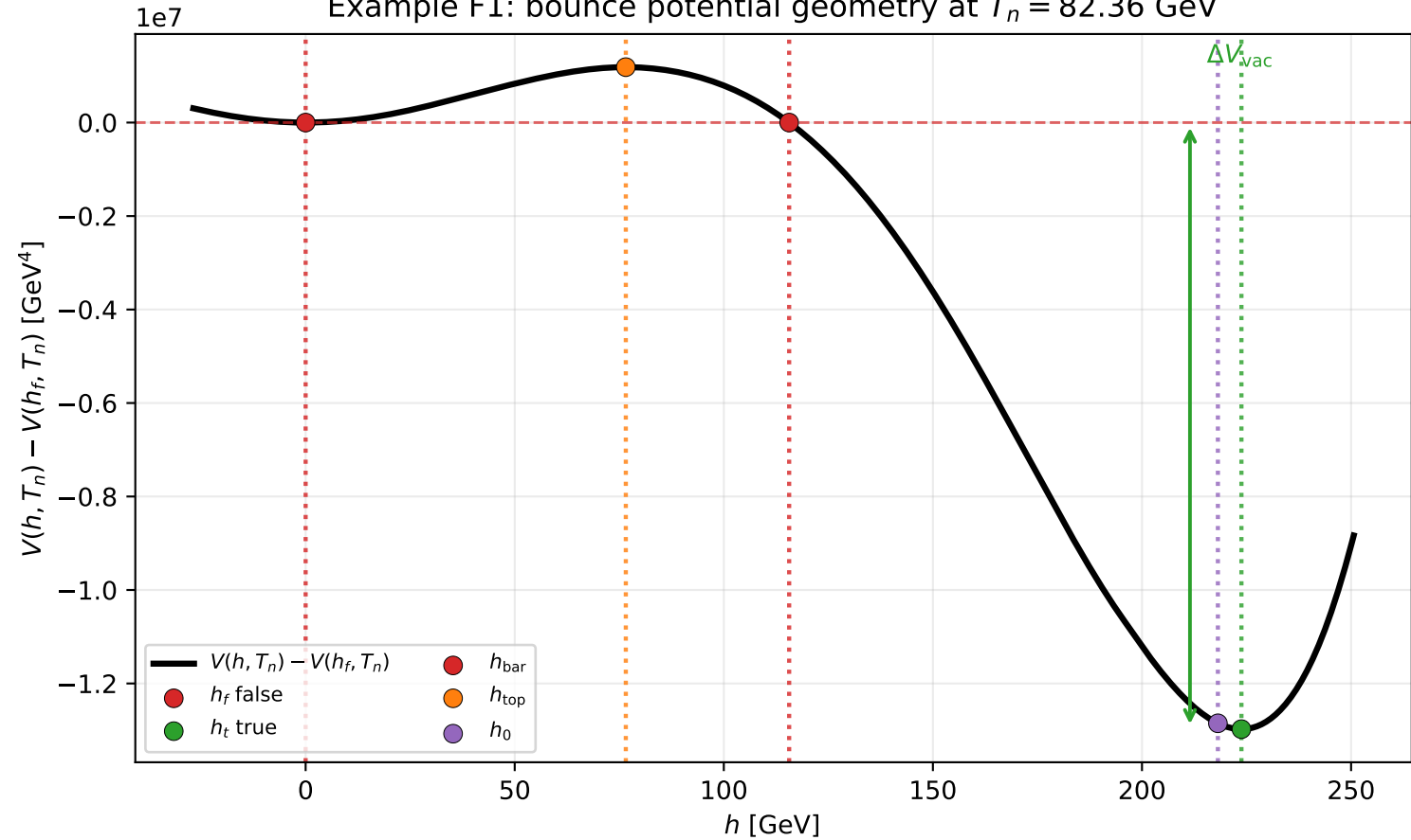
Example F1: bounce potential geometry at T_n = 82.36 GeV
