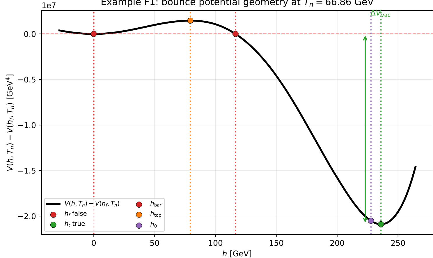
Example F1: bounce potential geometry at T_n = 66.86 GeV
