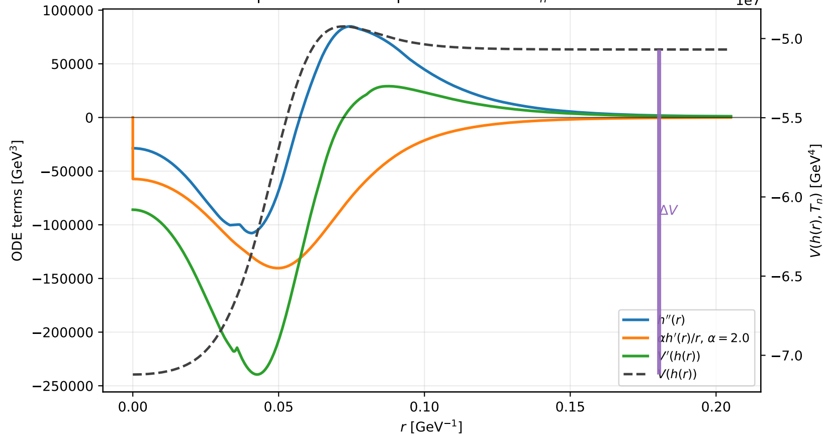
Example F7: bounce equation terms at T_n = 66.86 GeV
