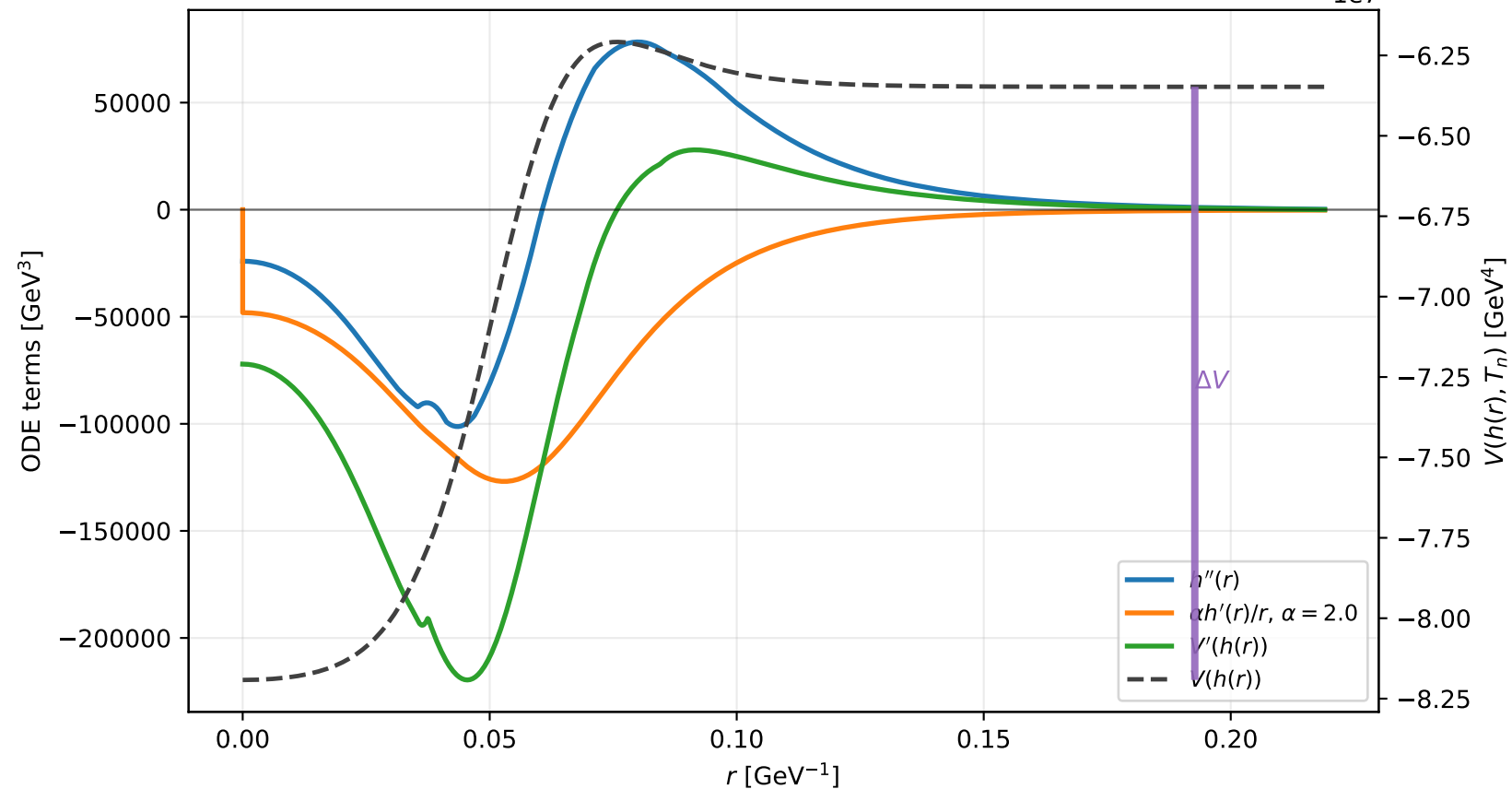
Example F7: bounce equation terms at T_n = 70.68 GeV
