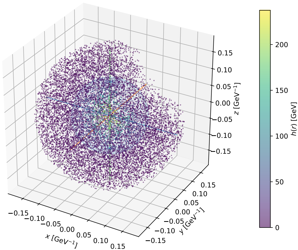
Example F5: 3D bubble profile at T_n = 64.13 GeV
