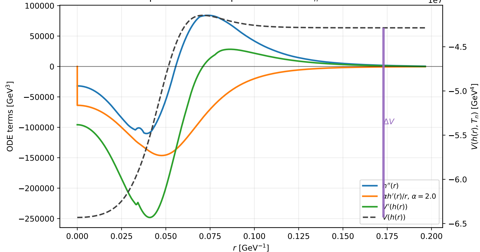
Example F7: bounce equation terms at T_n = 64.13 GeV
