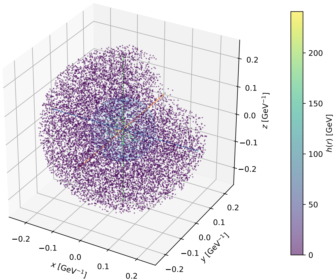
Example F5: 3D bubble profile at T_n = 56.89 GeV
