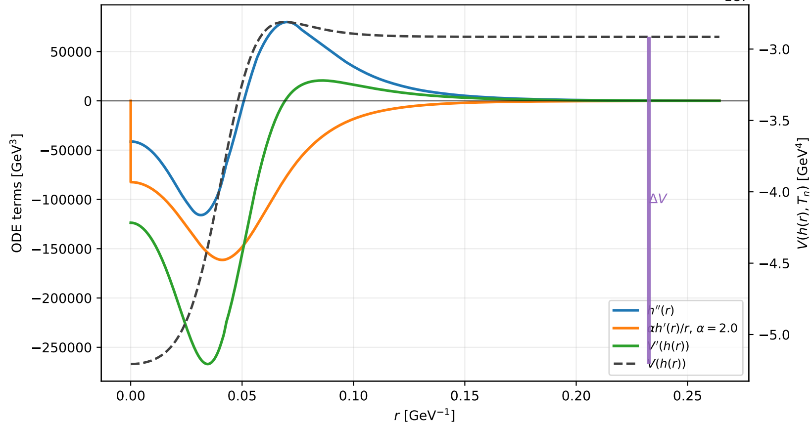
Example F7: bounce equation terms at T_n = 56.89 GeV
