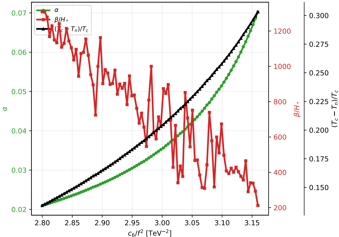
Run 05: pure \phi^6 + \phi^8 scan: c_8/f^4 [TeV ^{-4} ]=5, with daisy
