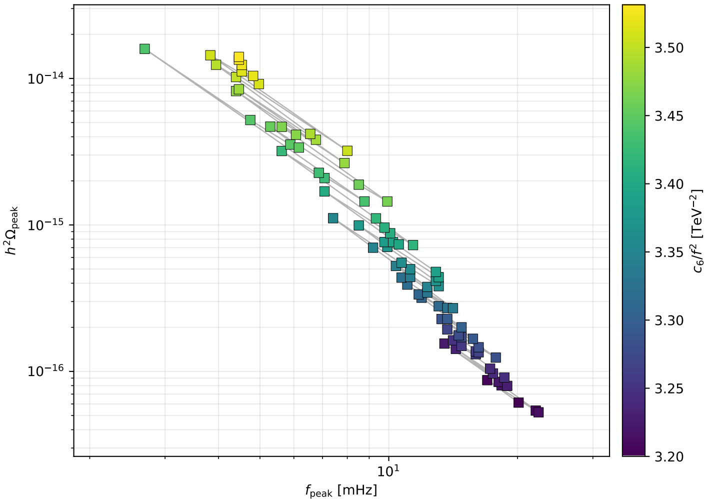
Run 05: pure \phi^6 + \phi^8 scan: peak motion, c_8/f^4 [TeV ^{-4} ]=0, with daisy
