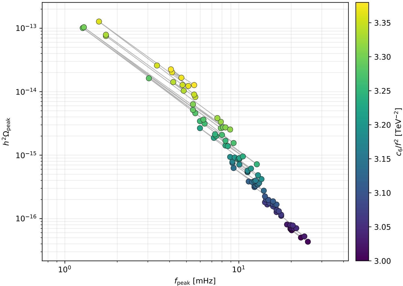
Run 05: pure \phi^6 + \phi^8 scan: peak motion, c_8/f^4 [TeV ^{-4} ]=2, no daisy
