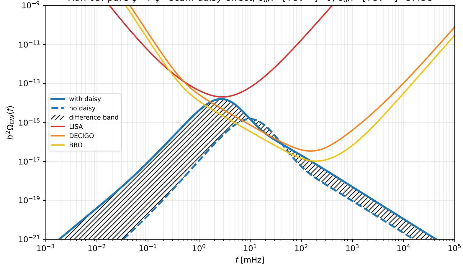
Run 05: pure \phi^6 + \phi^8 scan: daisy effect, c_8/f^4 [TeV ^{-4} ]=0, c_6/f^2 [TeV ^{-2} ]=3.438
