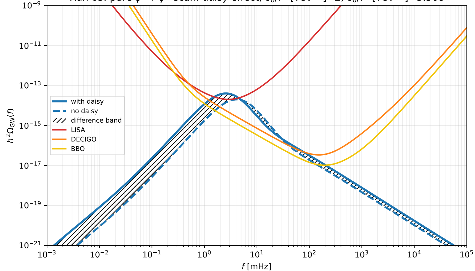
Run 05: pure \phi^6 + \phi^8 scan: daisy effect, c_8/f^4 [TeV ^{-4} ]=2, c_6/f^2 [TeV ^{-2} ]=3.368
