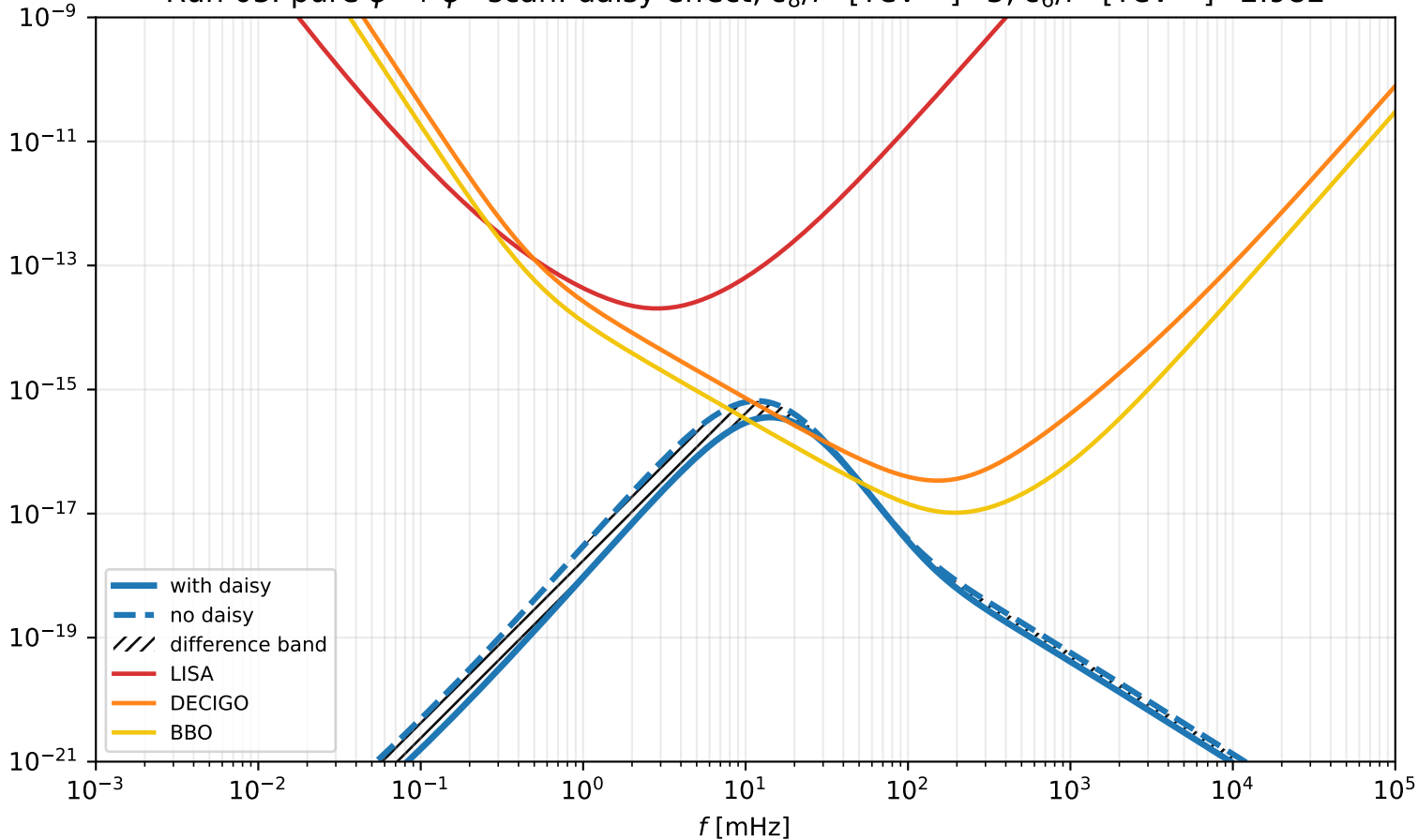
Run 05: pure \phi^6 + \phi^8 scan: daisy effect, c_8/f^4 [TeV ^{-4} ]=5, c_6/f^2 [TeV ^{-2} ]=2.982
