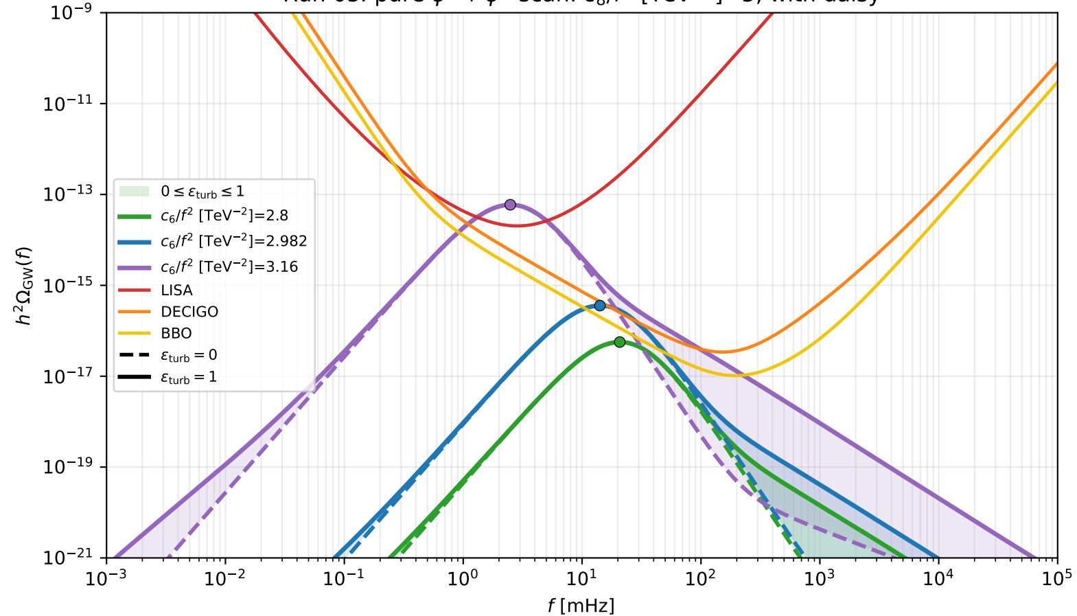
Run 05: pure \phi^6 + \phi^8 scan: c_8/f^4 [TeV ^{-4} ]=5, with daisy
