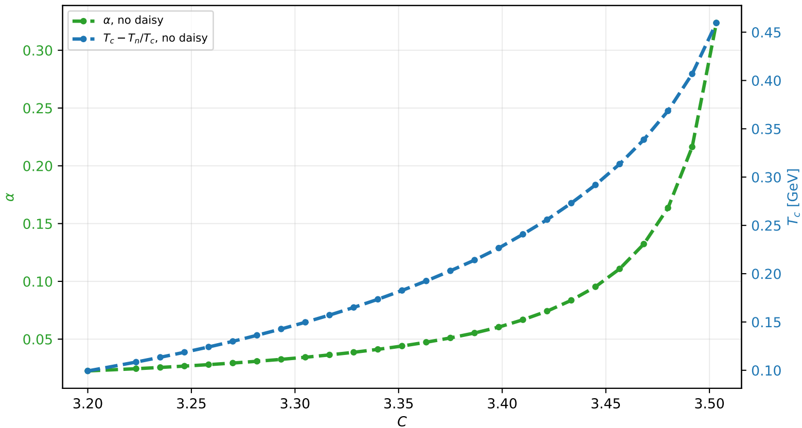
Run 06: combined \phi^6 + \phi^8 + Gláuber scan in C c_8/f^4 = 0 \text{ TeV}^{-4} , c_6/f^2 = 1 \text{ TeV}^{-2} , \Lambda = 1000 \text{ GeV} , f = 1000 \text{ GeV}
