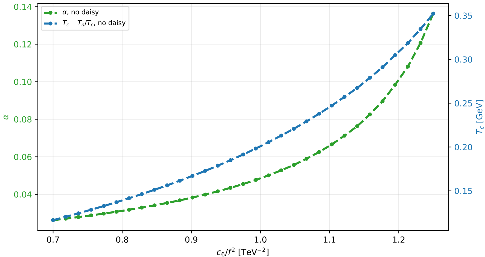
Run 07: combined \phi^6 + \phi^8 + Gláuber scan in c_6/f^2 c_8/f^4 = 5 \text{ TeV}^{-4} , C = 3.2 , \Lambda = 1000 \text{ GeV} , f = 1000 \text{ GeV}
