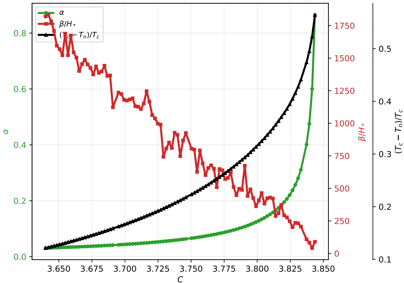
Run 03: pure Gláuber C scan: \Lambda [GeV]=1000, no daisy
