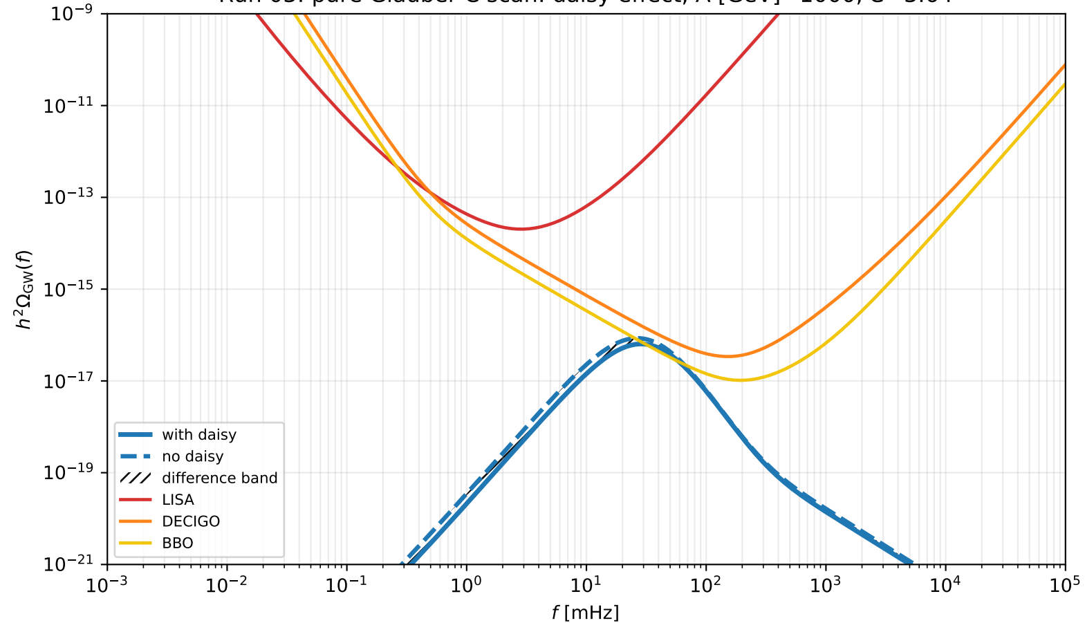
Run 03: pure Gláuber C scan: daisy effect, \Lambda [GeV]=1000, C=3.64
