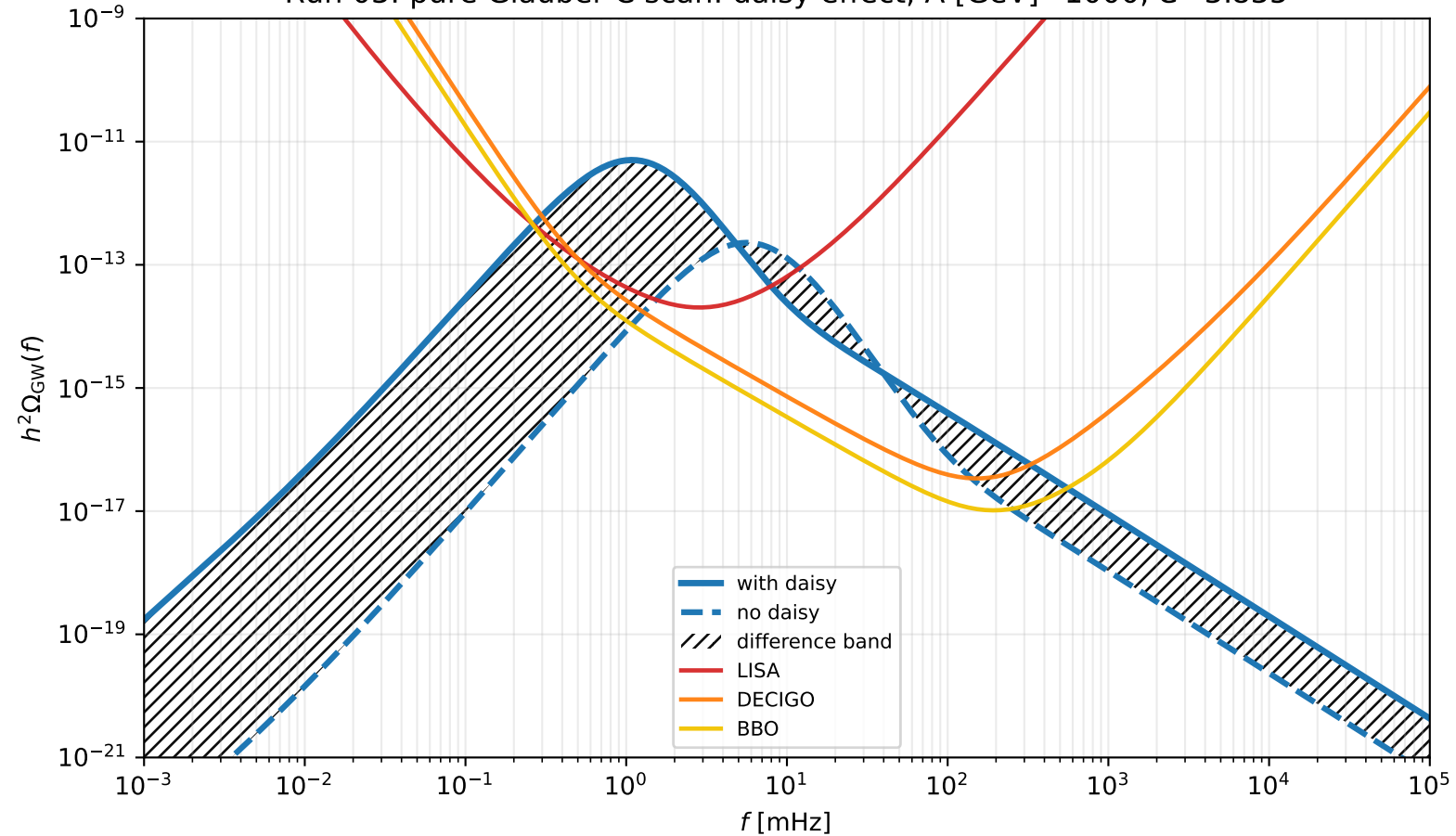
Run 03: pure Gláuber C scan: daisy effect, \Lambda [GeV]=1000, C=3.835
