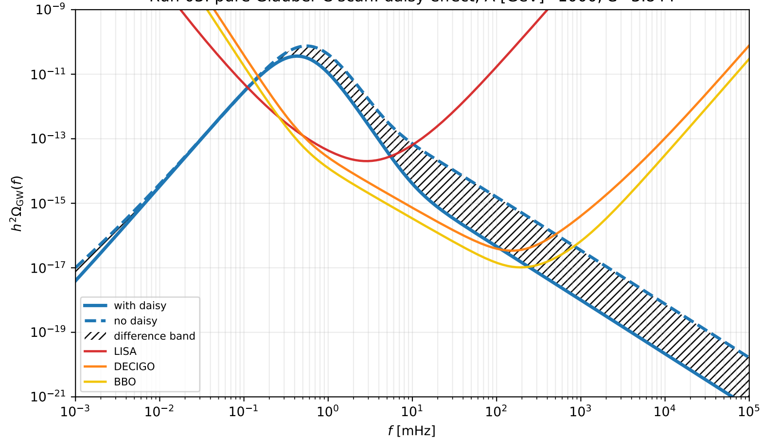
Run 03: pure Gláuber C scan: daisy effect, \Lambda [GeV]=1000, C=3.844
