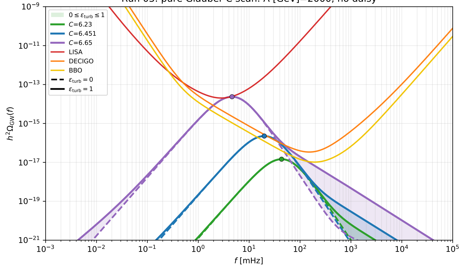
Run 03: pure Gláuber C scan: \Lambda [GeV]=2000, no daisy
