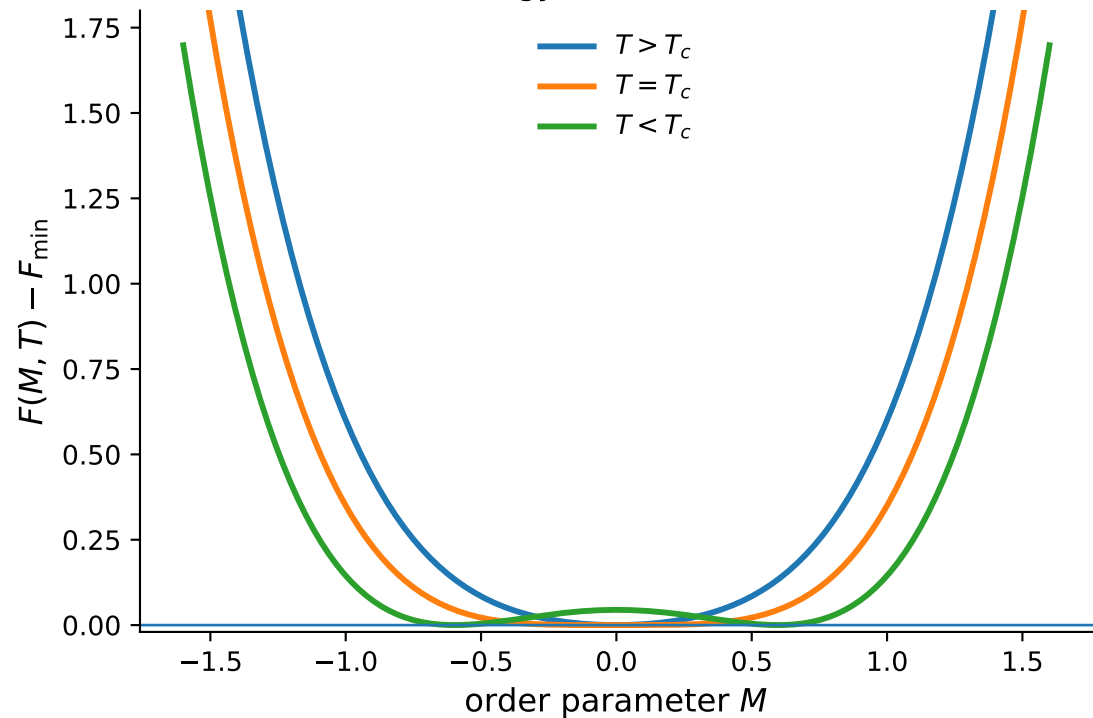
Landau free energy for a continuous transition
