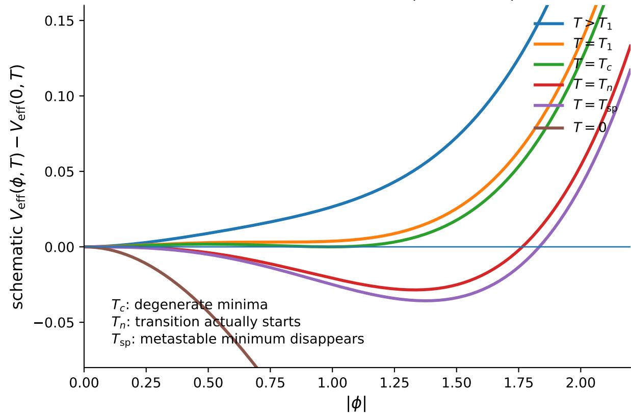
Schematic first-order transition: important temperatures
