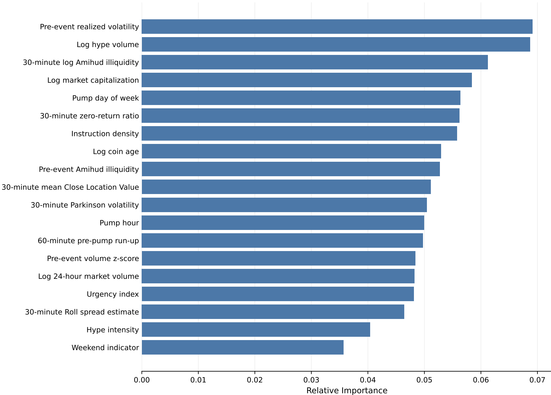
Feature Importance for Predicting Pump Success (XGBoost)
