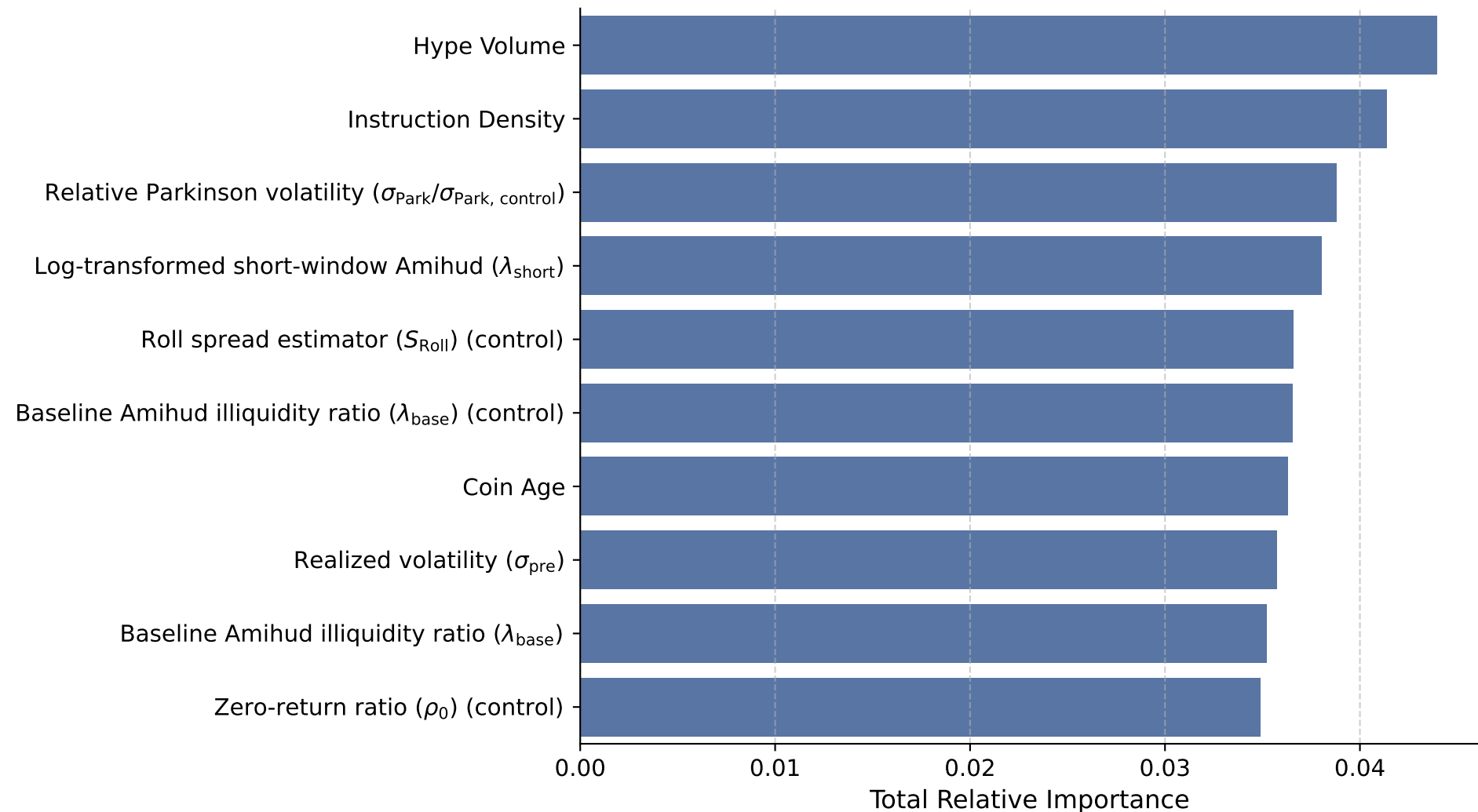
Top Drivers of Pump Success (Aggregated | XGBoost)
