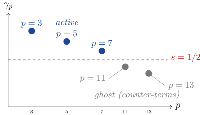
Figure 1: Anomalous dimensions \gamma_p(15) for the first five odd primes. The threshold s = 1/2 (dashed red) separates the three active primes (blue circles) from the ghost primes (gray circles).
