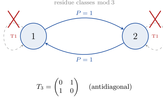
Figure 1.2: Transition graph of the mod-3 sieve dynamics. Sieve candidates alternate between residue classes 1 and 2 with probability 1. Self-transitions are absolutely forbidden (T1, red crosses). The transfer matrix T_3 is purely antidiagonal—the simplest non-trivial dynamical law.
