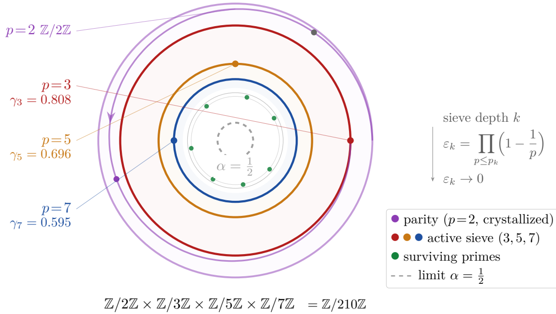
Figure 1.4: The prime sieve as a converging spiral. The integers n = 1, \dots, 210 are mapped onto the spiral via t = n/210 (one full CRT period, 210 = 2 \times 3 \times 5 \times 7 ). The outermost shell ( p = 2 , purple) removes all even integers (parity crystallization); successive shells for p = 3 (red), 5 (orange), 7 (blue) further narrow the surviving region. Green dots mark surviving primes within one period. The dashed circle is the asymptotic limit \alpha = 1/2 .
