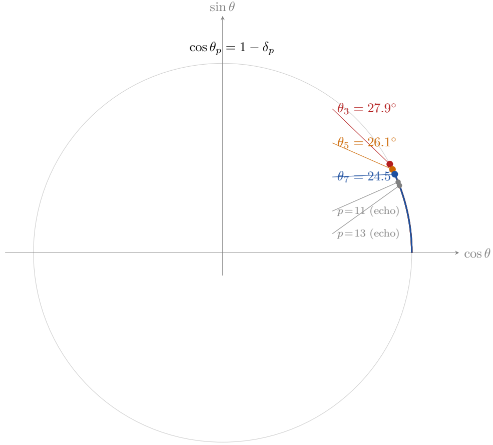
Figure 7.2: Cyclic Phase angles on the unit circle. Each active prime p \in \{3, 5, 7\} defines an angle \theta_p via \cos \theta_p = 1 - \delta_p . The squared sine \sin^2 \theta_p is the coupling strength. Inactive primes ( p \geq 11 , gray) lie closer to the axis.
