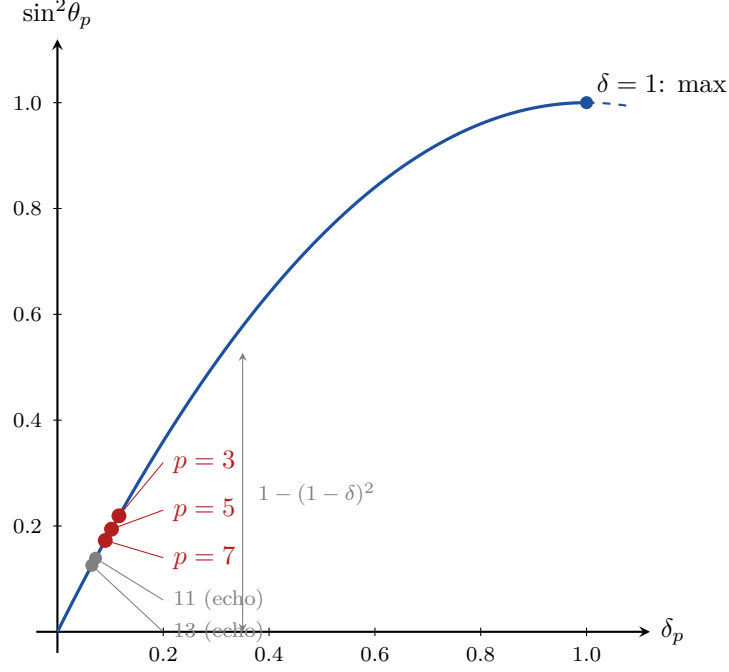
Figure 7.1: Cyclic Phase parabola \sin^2 \theta_p = \delta_p(2 - \delta_p) . Red dots: active primes \{3, 5, 7\} at q_+ = 13/15 . Gray dots: inactive primes \{11, 13\} . The three active primes cluster near \delta \approx 0.1 , where \sin^2 \theta_p \approx 2\delta_p (linear regime).
