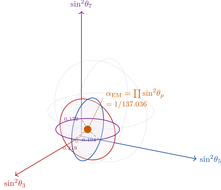
Figure 7.4: The coupling sphere. Each axis represents \sin^2 \theta_p for one active prime. Three coloured circles, each perpendicular to one axis, intersect at the unique point (\sin^2 \theta_3, \sin^2 \theta_5, \sin^2 \theta_7) whose product equals \alpha_{\text{EM}} = 1/137.036 . The coupling point lies deep in the low- \theta region: nature uses only a small fraction of the available parameter space.
