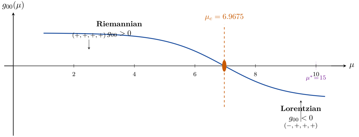
Figure 22.2: Lorentzian signature transition. The metric component g_{00}(\mu) = -d^2(\ln \alpha_{\text{EM}})/d\mu^2 changes sign at the critical scale \mu_c = 6.9675 . For \mu > \mu_c (including \mu^* = 15 ), the Fisher geometry acquires Lorentzian signature (-, +, +, +) : time emerges from information curvature.
