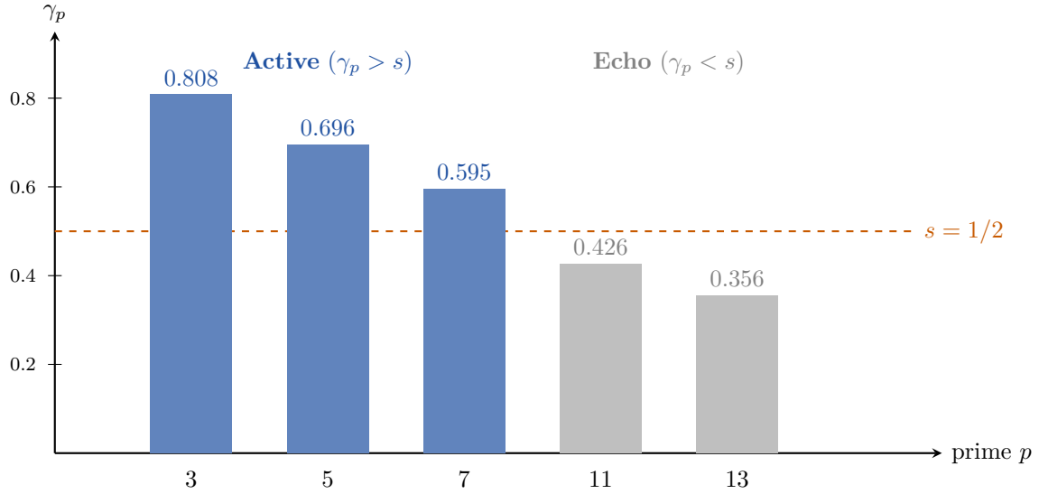
Figure 7.3: Anomalous dimensions \gamma_p at \mu^* = 15 . The threshold \gamma_p = s = 1/2 (orange dashed) separates the three active primes \{3, 5, 7\} (blue) from the echo primes \{11, 13, \dots\} (gray). This determines N_c = 3 .
