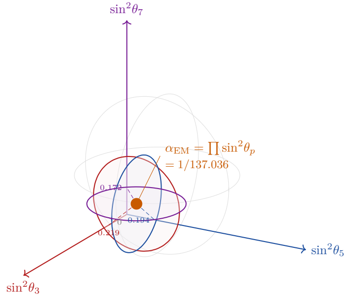
Figure 7.6: The coupling sphere. Each axis represents \sin^2\theta_p for one active prime. Three coloured circles, each perpendicular to one axis, intersect at the unique point (\sin^2\theta_3, \sin^2\theta_5, \sin^2\theta_7) whose product equals \alpha_{EM} = 1/137.036 . The coupling point lies deep in the low- \theta region: nature uses only a small fraction of the available parameter space.
