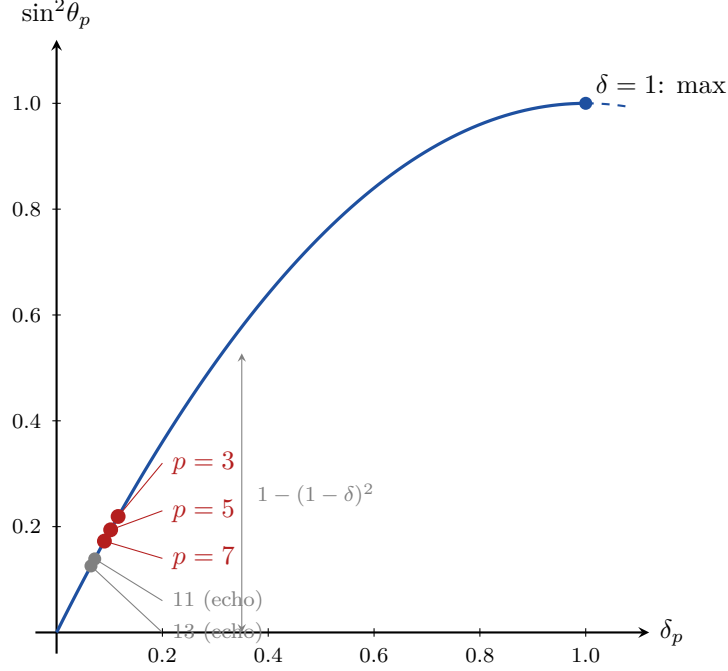
Figure 7.3: Cyclic Phase parabola \sin^2\theta_p = \delta_p(2 - \delta_p) . Red dots: active primes \{3, 5, 7\} at q_+ = 13/15 . Gray dots: inactive primes \{11, 13\} . The three active primes cluster near \delta \approx 0.1 , where \sin^2\theta_p \approx 2\delta_p (linear regime).
