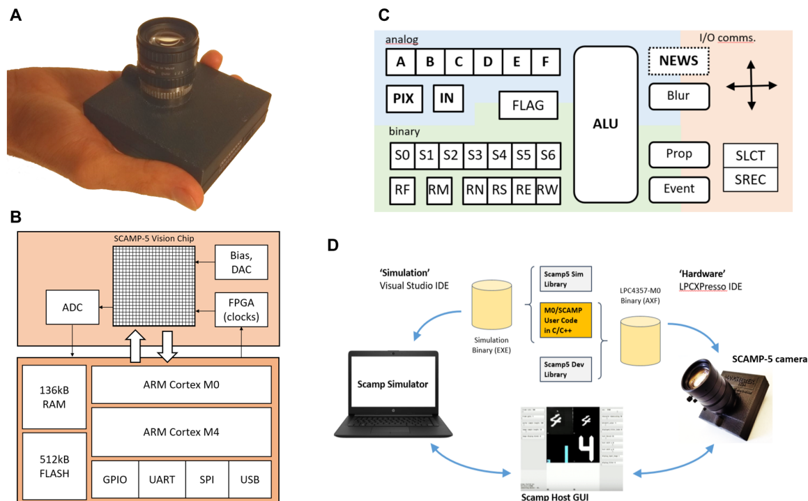
Fig. 5. SCAMP-5 smart camera system, used in many of the applications reported here. (A) Prototype camera. (B) System architecture. At the core of the system is the SCAMP-5 vision chip comprising an array of 256 \times 256 processing elements, control, and readout circuits. The camera integrates peripheral circuitry including biasing, clocking, analog/digital converters, and MCU comprising two 32-bit processor cores, memory, and interfaces. (C) Architecture of the processing element on the SCAMP-5 chip. It includes analog and binary registers, some special-purpose registers, arithmetic logic unit, interface, and control circuitry; processors communicate directly with four nearest neighbors. (D) Software development and debugging tools, including system simulator and user interface, enable construction of libraries of useful image processing functions that can be then joined into a complete vision application.
