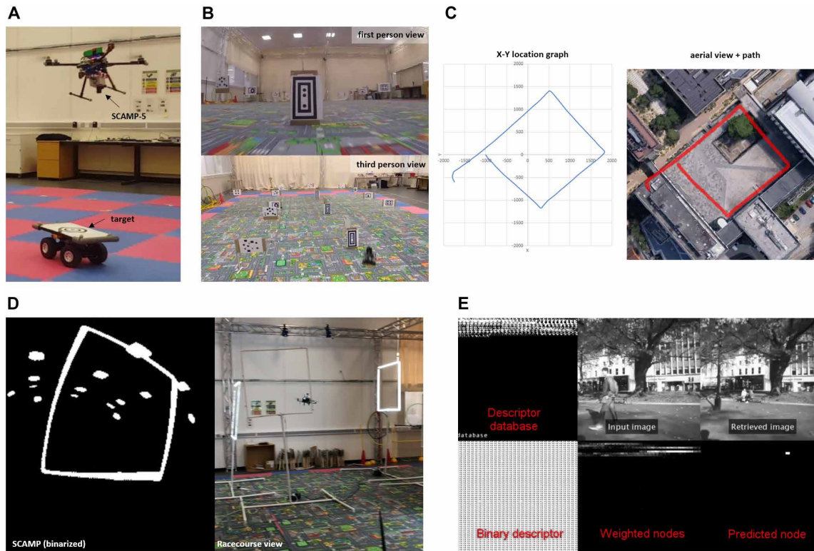
Fig. 7. Robotic applications with PPAs. (A) Closely tracking a mobile target that follows unpredictable chaotic paths with a quadrotor. (B) An agile nonholonomic vehicle makes decisions at 2000 fps on navigation trajectories based on visual targets when traveling at 4 m/s. (C) VO on a PPA at 1000 fps. (D) A quadrotor with a PPA estimates gate pose to fly through on a drone race course. (E) Pictorial mapping and localization on the focal plane. Inset shows (left to right and top to bottom) pictorial map, input image, retrieved image, input image descriptor representation, weighted location nodes, and predicted location node.
