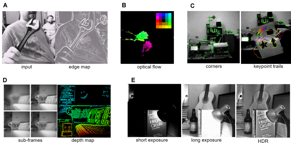
Fig. 6. Image processing algorithms executed on the SCAMP-5 PPA. (A) Sobel edge detection. Execution time is 5.8 \mu s. (B) Optical flow. Image shows two objects moving in different directions, and inset shows directional color coding. A block-matching algorithm using 5 by 5 blocks matched over 5 by 5 grid takes \sim 0.4 ms. (C) Corner detection using FAST-16 algorithm. Keypoint trails show past keypoints; the test card was rotating. Images are output for illustration. When outputting only keypoint coordinates, the system can operate at 2000 fps (68). (D) Depth from focus. Subframes are acquired by sweeping the focus of a liquid lens at 60 Hz, and up to 128 subframes are processed to determine a combined depth map at 60 fps. In the image, red is near, and blue is far; this requires a spatial contrast maximization algorithm running at 7000 fps (67). (E) High dynamic range imaging using tone mapping by combining hundreds of frames. The image is progressively exposed to achieve locally balanced image intensity at each pixel (66).
