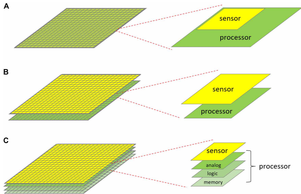
Fig. 4. Pixel-parallel vision sensors in 3D stacked technologies. (A) In a standard planar CMOS technology, sensors and processors share pixel area in a 2D space. (B) Current Cu–Cu wafer bonding technologies allow placing processor circuitry underneath the image sensor. The light-sensitive area is maximized, whereas overall pixel size is reduced. (C) Advanced 3D stacking technologies may allow the distribution of in-pixel processors over multiple silicon tiers. Each tier could be fabricated using process technology optimized for sensing, analog circuits, digital logic, memory, etc.
