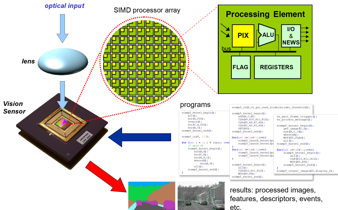
Fig. 3. PPA. Each pixel of the vision sensor device incorporates a processing element, including photosensor circuit (PIX), and a microprocessor-like datapath, including local memories (REGISTERS), arithmetic logic unit (ALU), local communications (NEWS), input/output (I/O) circuits, and local activity control (FLAG). The processing elements execute software programs, carrying out image computations on-sensor and outputting high-level information to the rest of the system.
