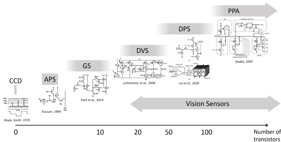
Fig. 2. Pixel-level circuits in image sensor devices. CCD image sensor pixels are transistor less (104), early CMOS image sensor pixels contained 1 transistor, modern active pixel sensor (APS) CMOS devices include three to four transistors per pixel (2), global shutter (GS) sensors contain up to 10 transistors (4), DVS devices include 15 to 30 transistors per pixel (7, 8), digital pixel sensors (DPS) include around 100 transistors in ADC converters and memory in each pixel (5, 6), vision sensors include 20 to 500 transistors in a processing circuit per pixel (16–25), and PPAs contain pixel-level processors including 150+ transistors (31–33, 48, 49).
