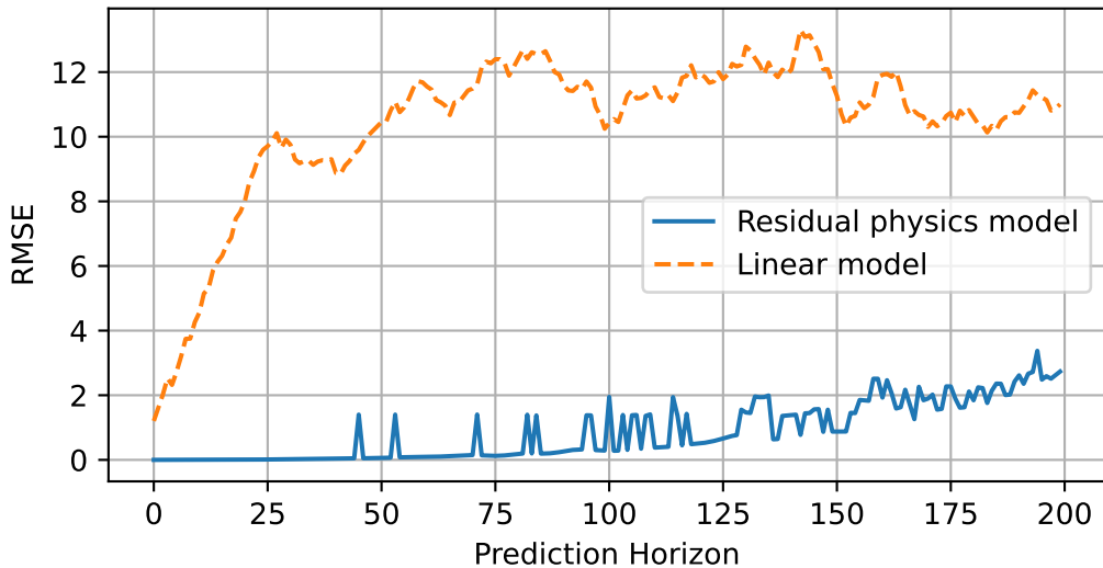
Multi-Step Rollout Prediction (200-step horizon)
