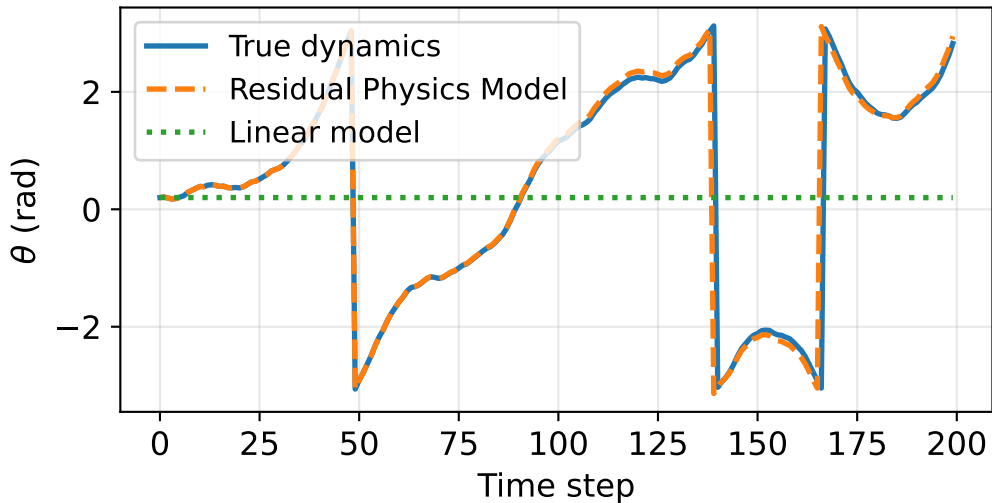
Trajectory Comparison of Identified Models
