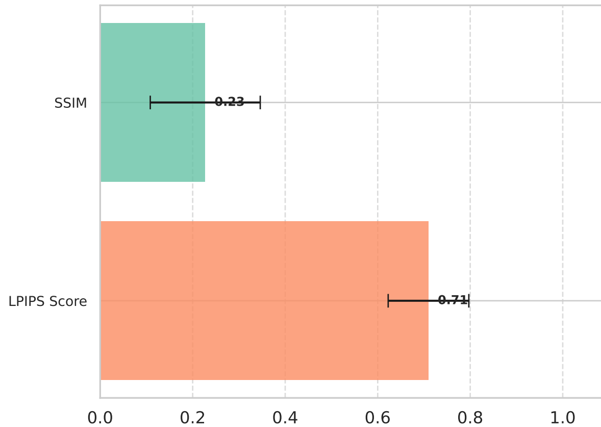
Edges & Boundaries
