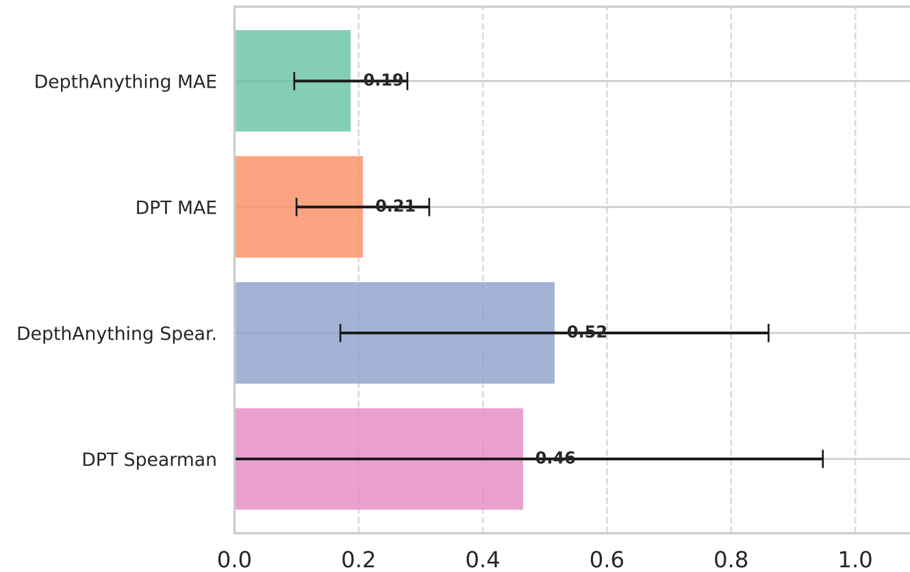
Depth & Geometry
