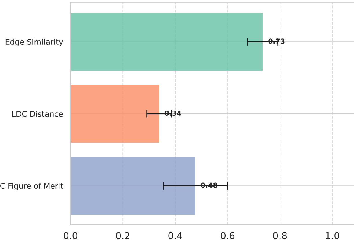
Edges & Boundaries
