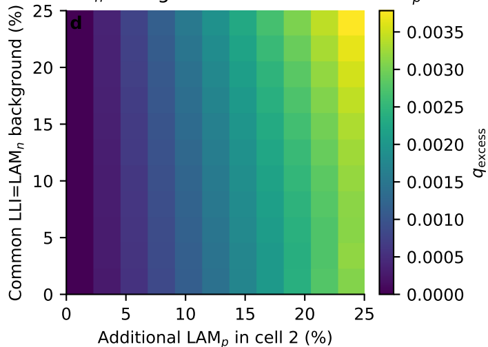
LLI+ \text{LAM}_n background + differential \text{LAM}_p
