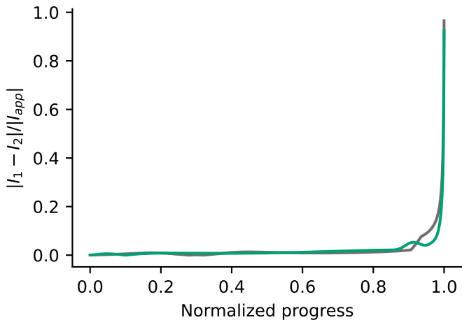
5% LLI+5% LAMn vs 10%+10%
