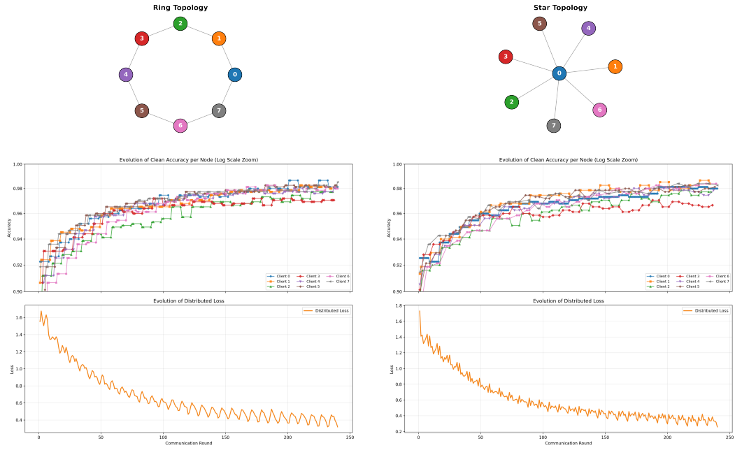
Figure A.2: Baseline performance comparison between the sparse Ring topology (left) and the centralized Star topology (right).
