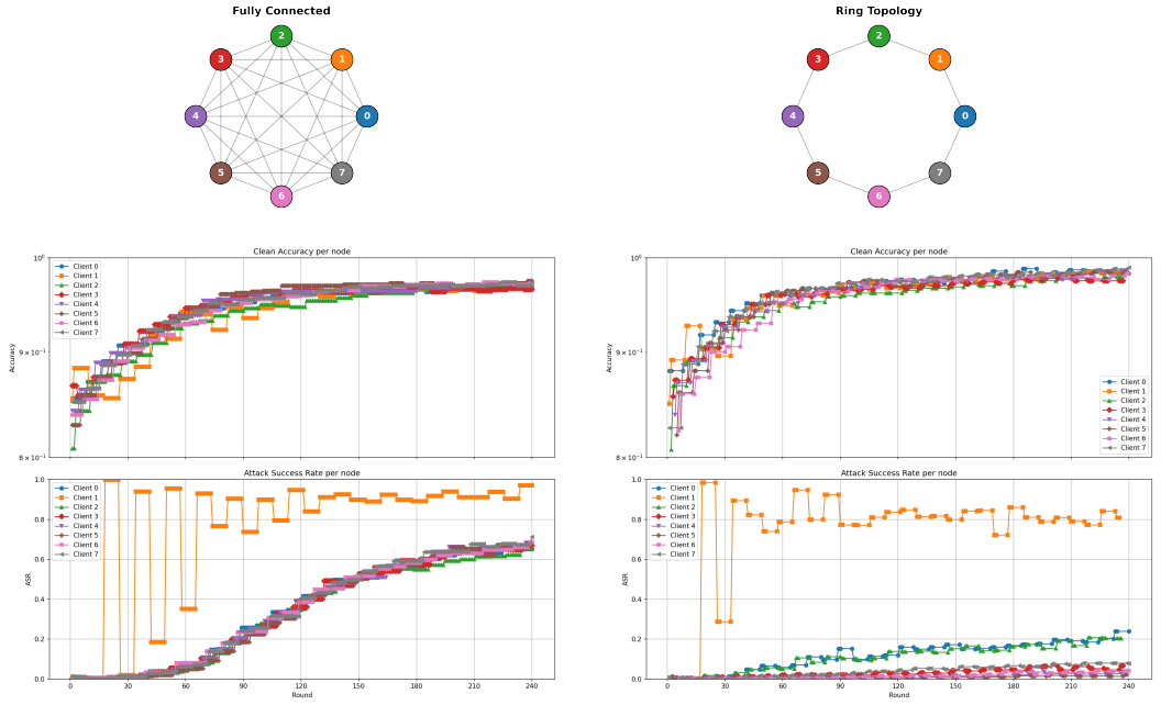
Figure A.4: Adversarial evaluation comparing a system-wide infection in the Fully Connected topology (left) against the staggered, sequential propagation delay inherent to the Ring topology (right). In both cases, the attacker is positioned at Client 1 (Orange).
