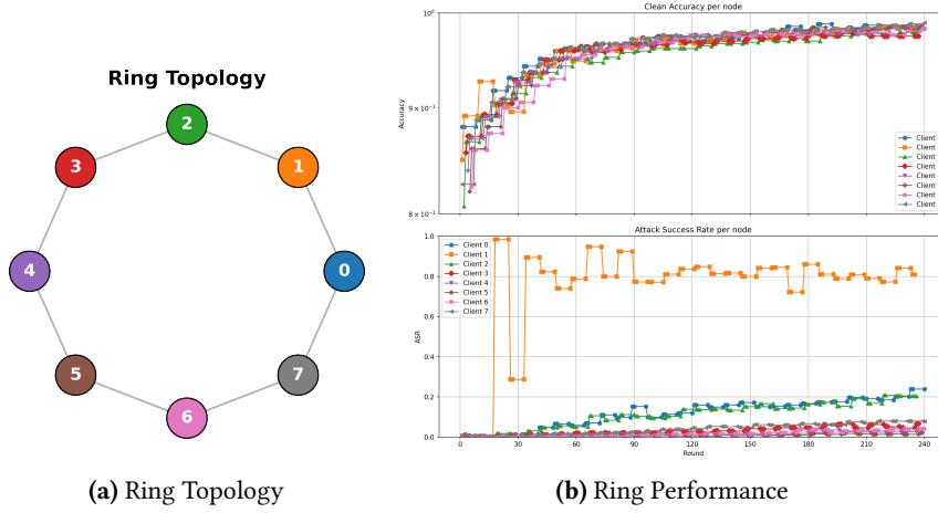
Figure 6.4: Evaluation of the Ring topology over 240 rounds. The staggered node infection is visually evident in the performance plot, corresponding to the topological distance from the attacker (Client 1).
