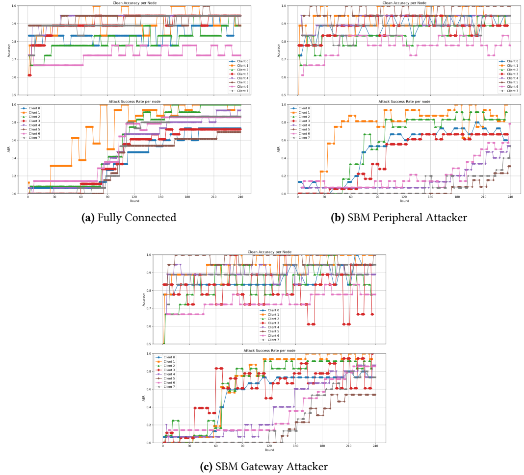
Figure 6.8: Clean Accuracy and ASR over 240 rounds for the NEU-DET dataset under three distinct topological configurations.
