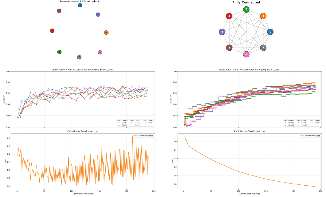
Figure A.1: Baseline performance comparison between the completely Isolated network (left) and the highly dense Fully Connected topology (right). The node colors in the graphs match the structural diagrams above.
