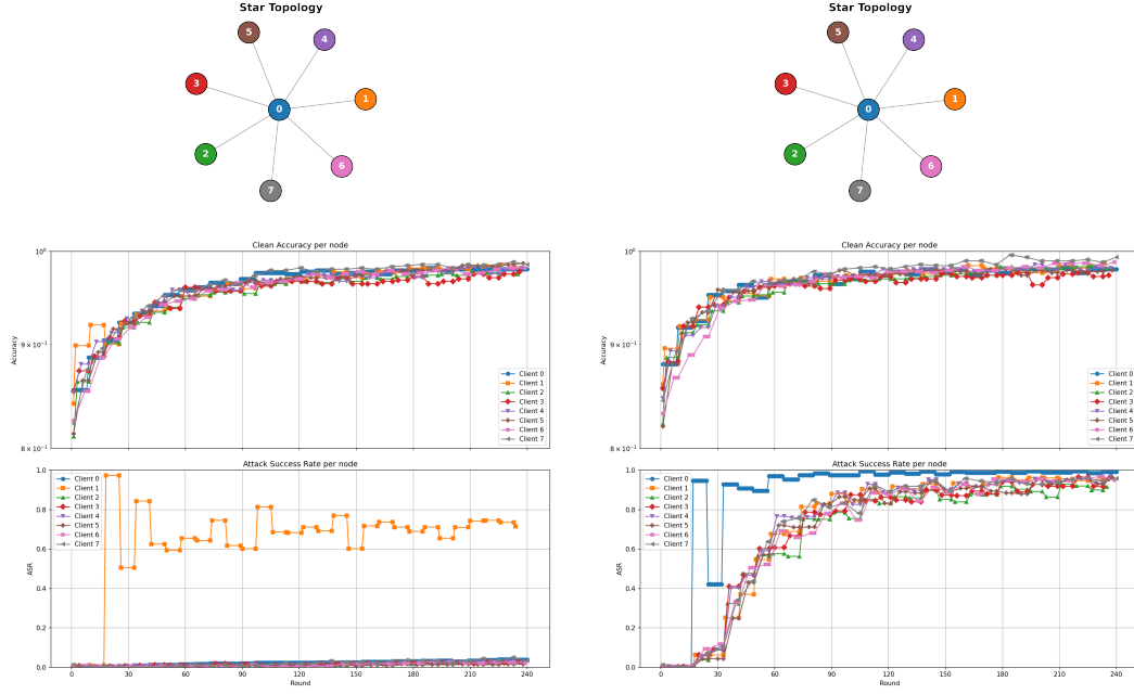
Figure A.5: Adversarial evaluation of the Star topology. A peripheral attacker (left, Client 1) is completely neutralized by the hub, whereas a compromised hub (right, Client 0) instantly corrupts the entire network.
