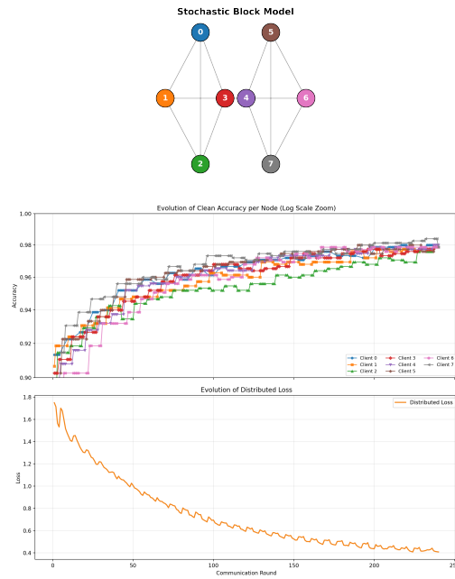
Figure A.3: Baseline performance for the Stochastic Block Model (SBM) topology, illustrating the natural convergence dynamics across two distinct communities.
