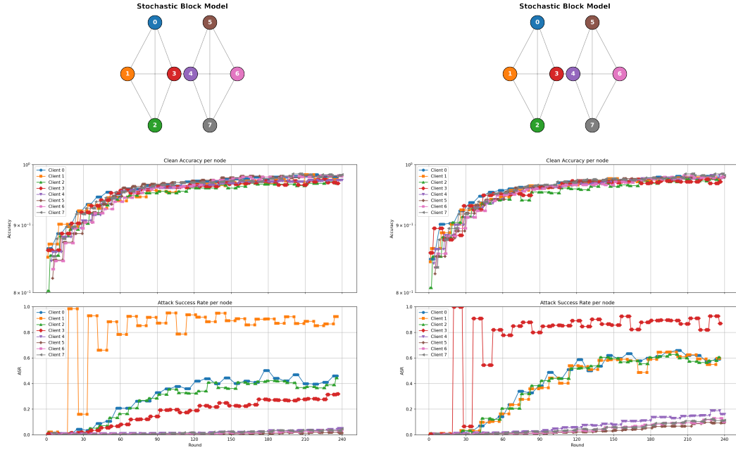
Figure A.6: Adversarial evaluation of the SBM topology. The structural bottleneck acts as a firewall against a peripheral infection (left, Client 1), and functions as a consensus sink to suppress an attack originating from the gateway itself (right, Client 3).
